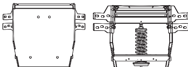
ALTERNATIVES SCHARNIER
