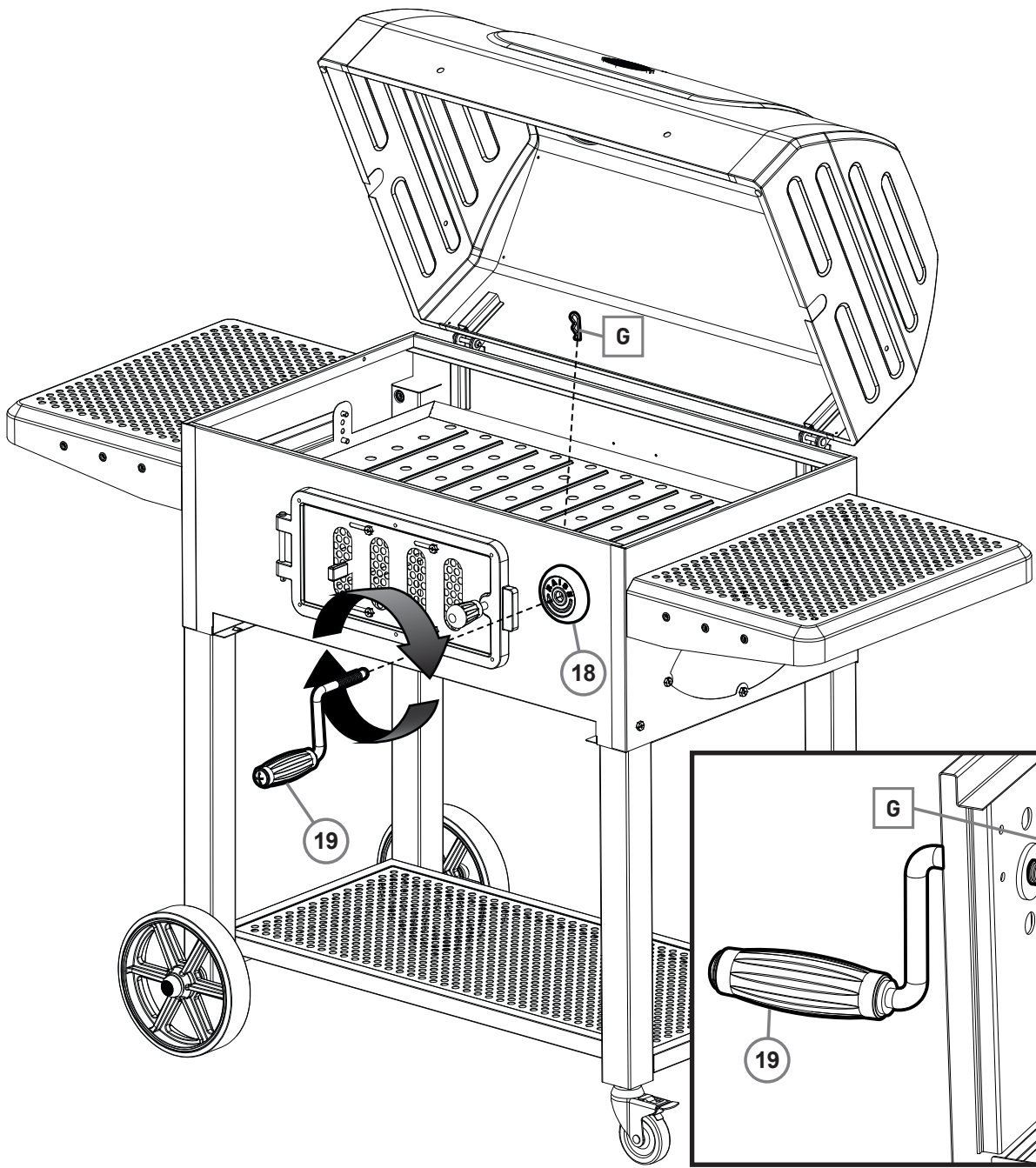
INTERIOR ASSEMBLED VIEW
