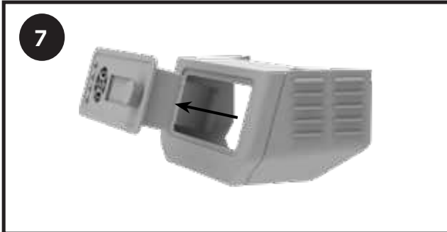
Pull the controller out of the failed housing.
