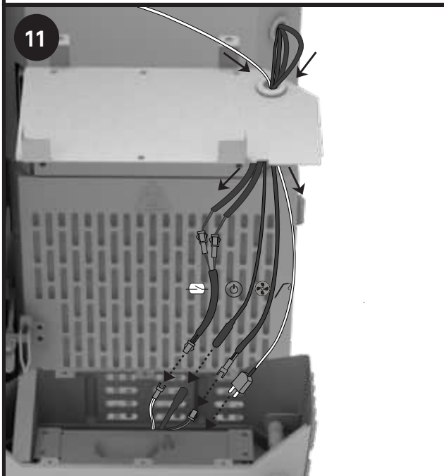
Pull the 4 wires into the hole and connect them.
