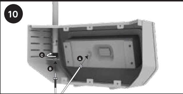
Reinstall the antenna and wire.
